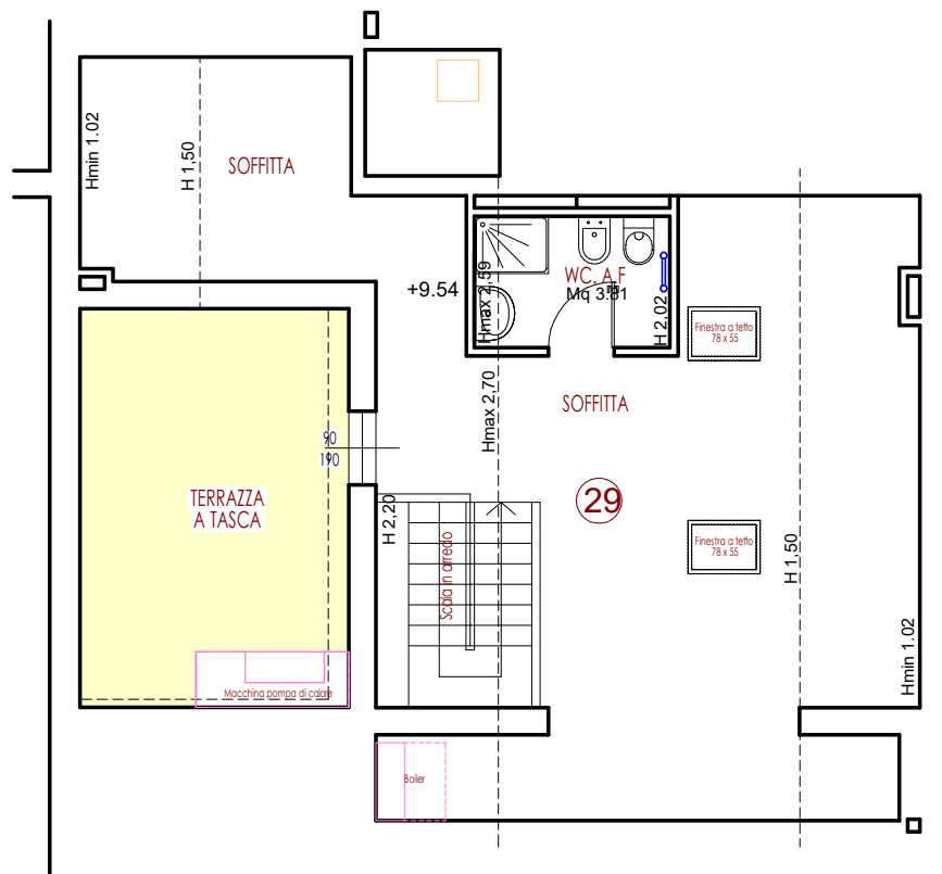
PIANO SOFFITTA
