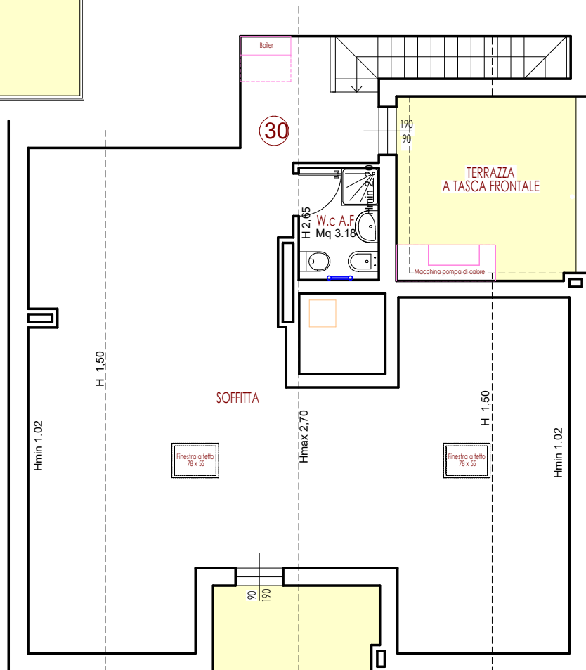
PIANO SOFFITTA
