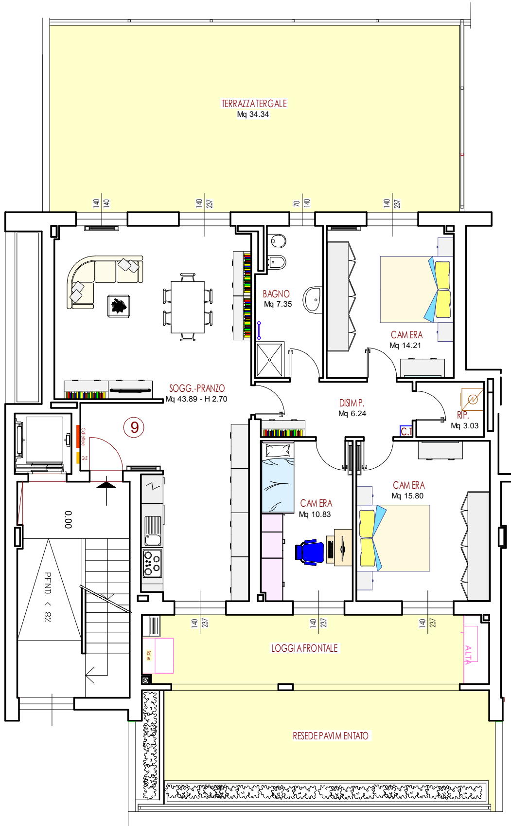
PIANO TERRA
